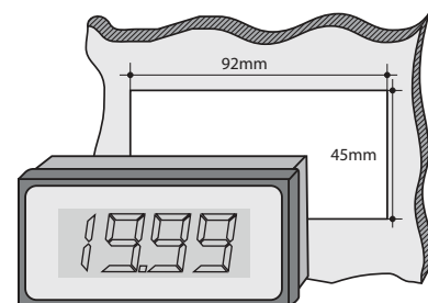
PANEL CUTOUT
